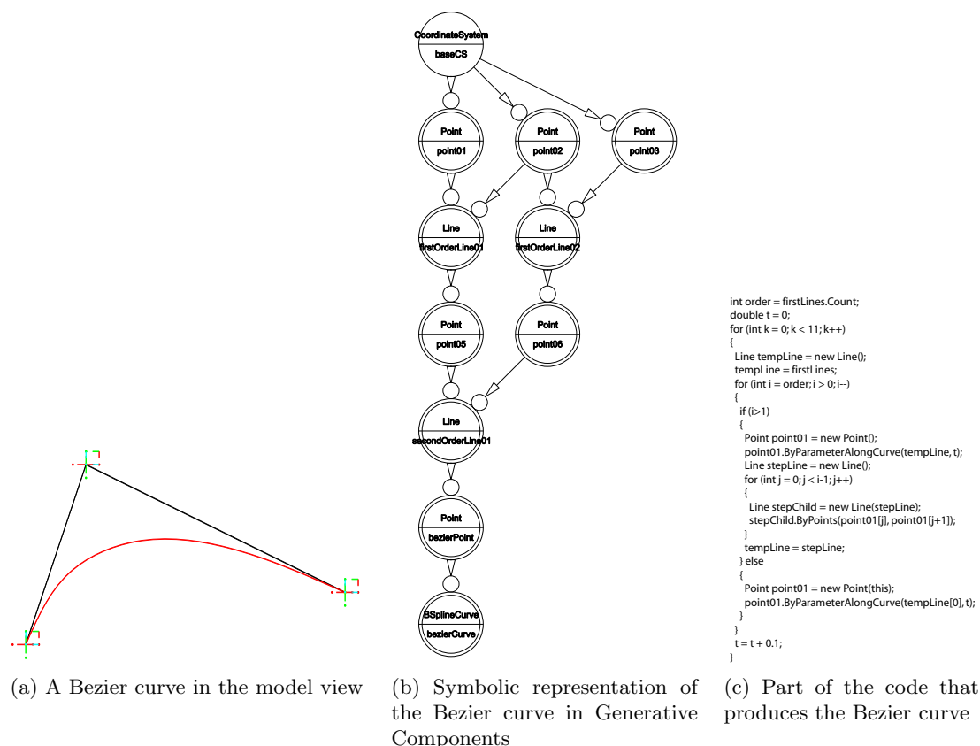
Figure F.4: Three representations of a Bezier curve in Generative Components
