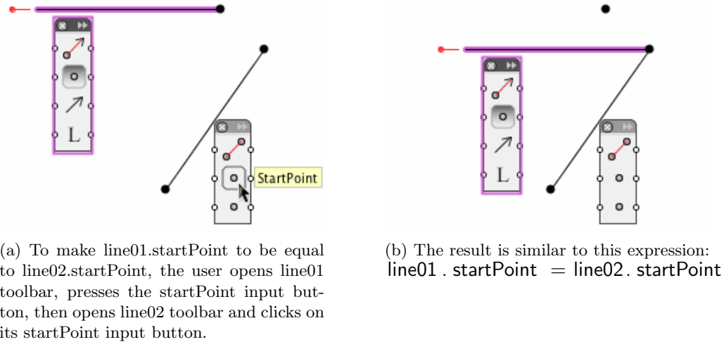
Figure 4.4: Accessing dot-notation properties of objects, using direct manipulation in the model.
